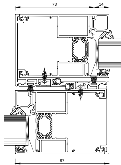
Section 2 STANDARD MEETING STILE
