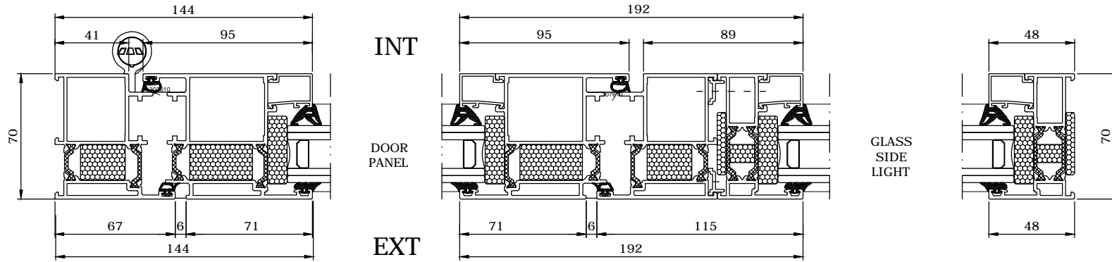
HORIZONTAL SECTION THROUGH DOOR PANEL AND FRAME WITH SIDELIGHT
