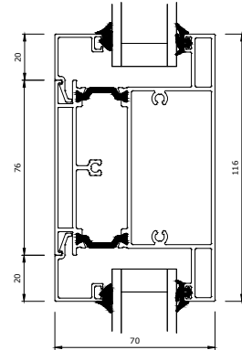
Optional Mid Rail
