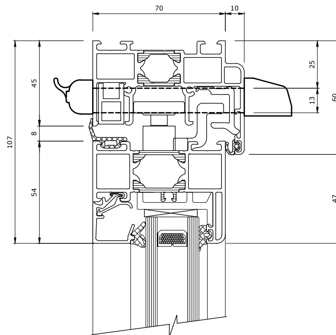
INTERNALLY OPENING
