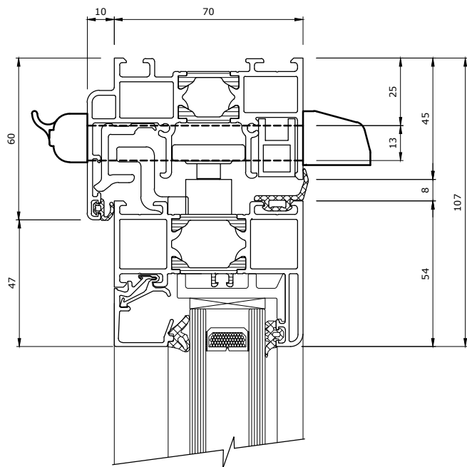
EXTERNALLY OPENING
